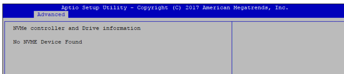
Figure 4-3-15: NVMe Configuration
