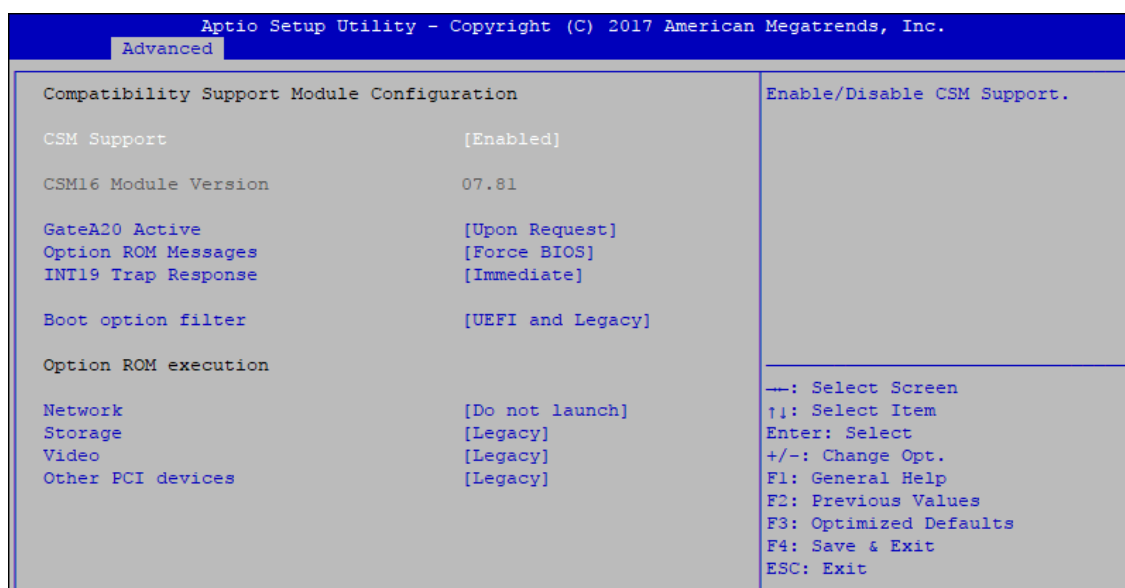
Figure 4-3-14: CSM Settings
