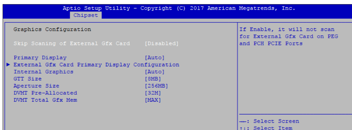
Figure 4-4-1-2: Graphics Configuration
