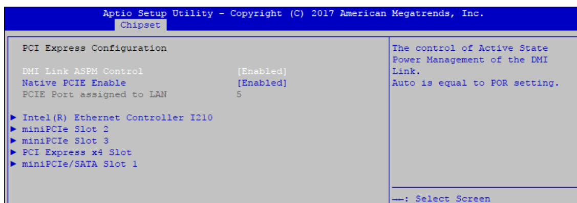
Figure 4-4-2-1: PCH-IO Settings
