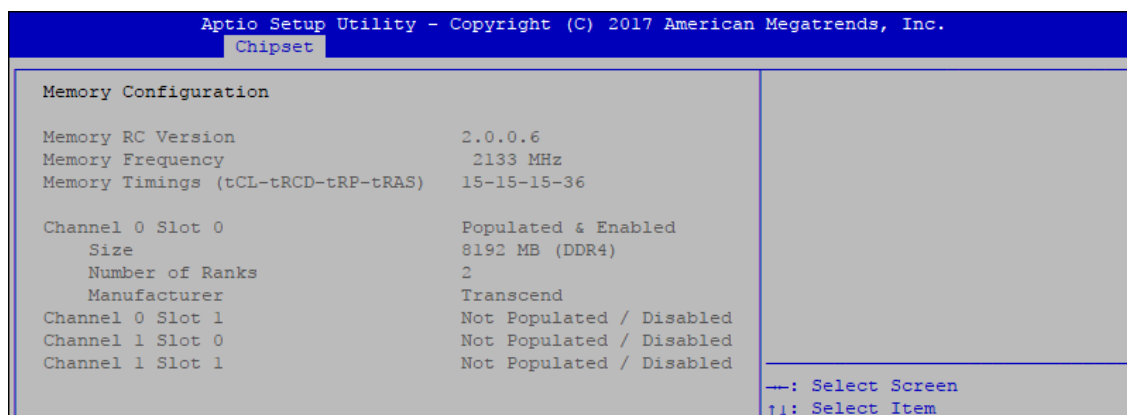
Figure 4-4-1-1: Memory Configuration
