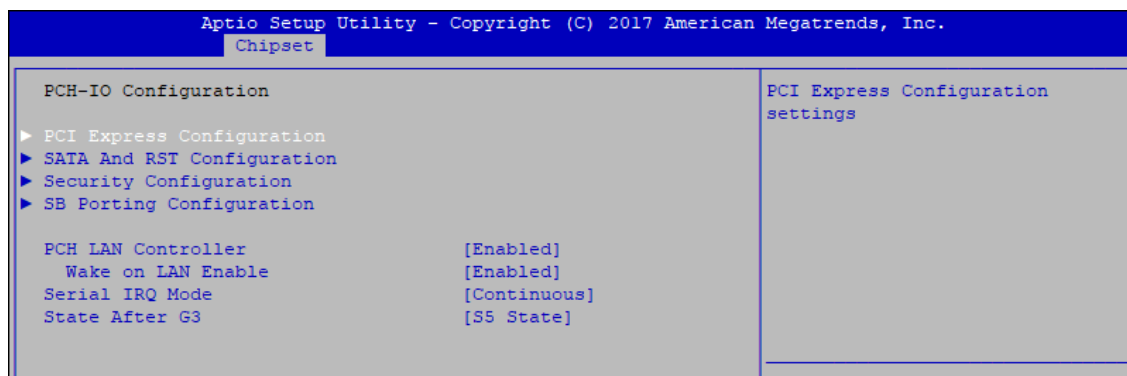
Figure 4-4-2: PCH-IO Settings
